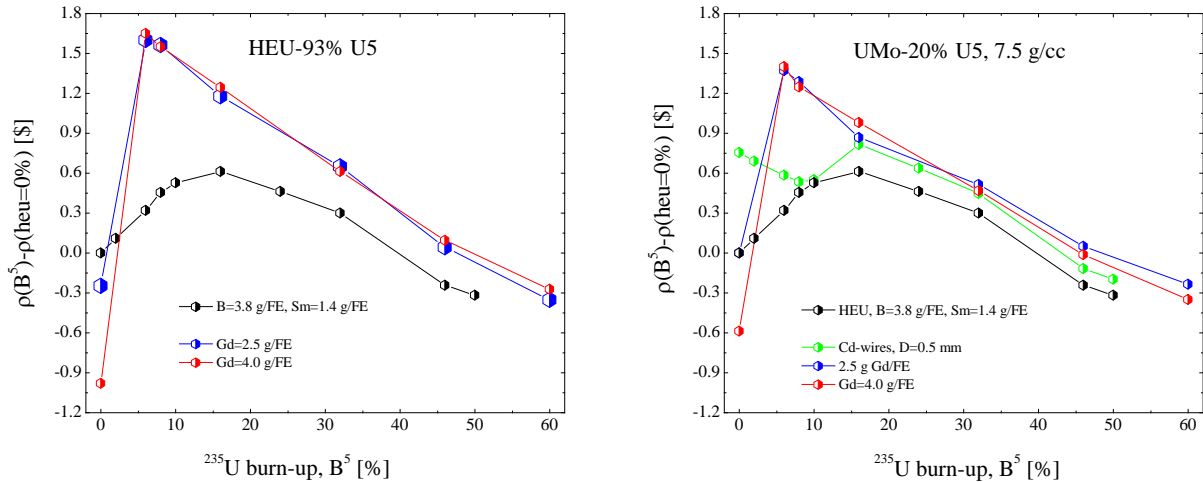
Figure 5. Performance graphs of reactivity of HEU & LEU fuel element vs. ^{235}\text{U} burn-up.
