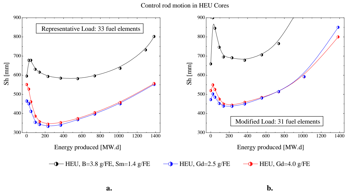
Figure 3. Control rod motion in HEU cores: a. representative load; b. modified load.
