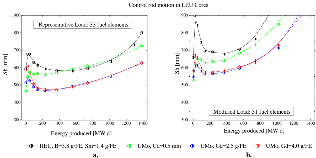
Figure 4. Control rod motion in LEU cores: a. representative load; b. modified load.
