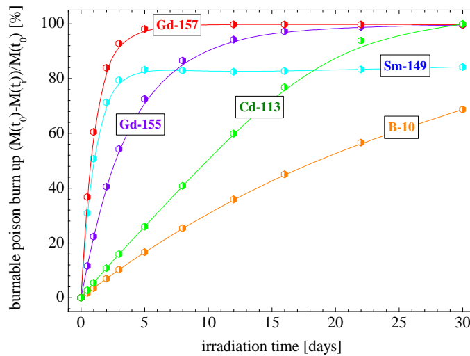
Figure 2. Comparison of burn up rate of different burnable poisons used in the HEU and LEU fuel assembly.
