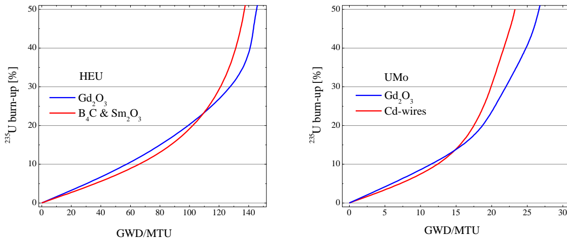
Figure 6. Increasing fuel element burn-up prior discharge by utilization of gadolinium as burnable absorber.
