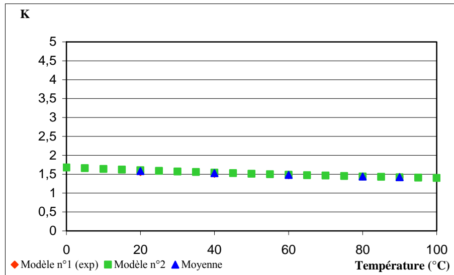
Figure 5.6 : DT + D_2O(l) \rightleftharpoons D_2 + DTO(l)
