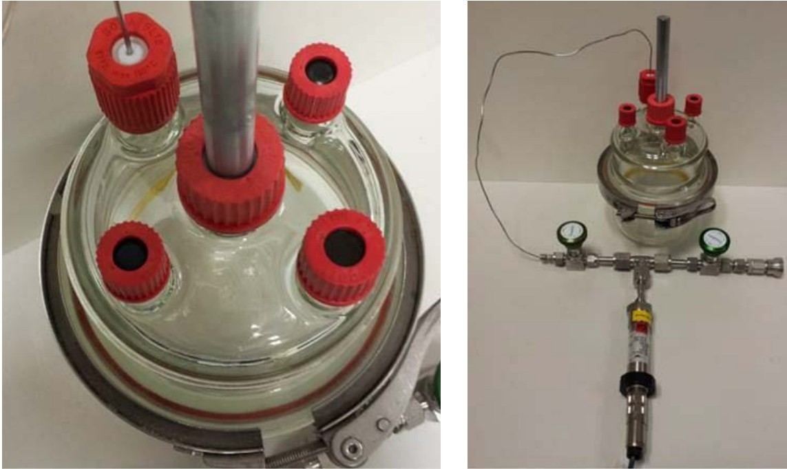
Figure 11. Accelerated corrosion test cell setup.
