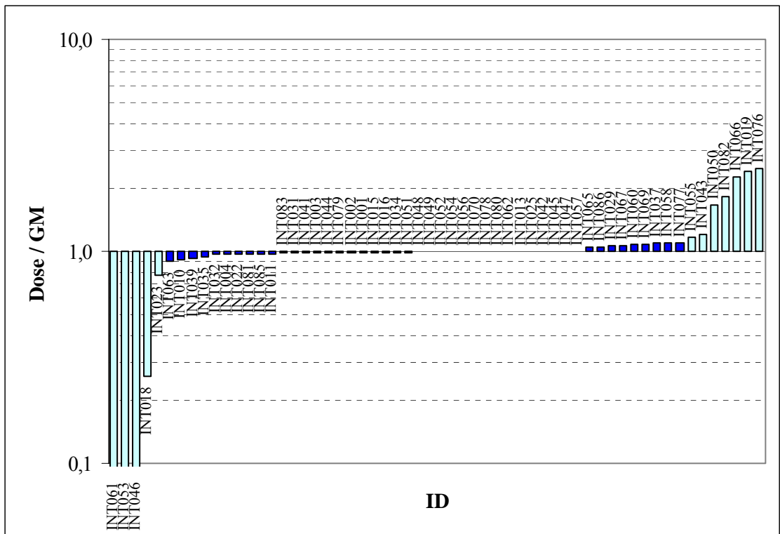
Figure 4-6. Results of the individual participants: Effective dose normalised to the geometric mean. (GM = 25.8 mSv, GSD = 1.06, N=47) The light blue bars represent the outliers.
