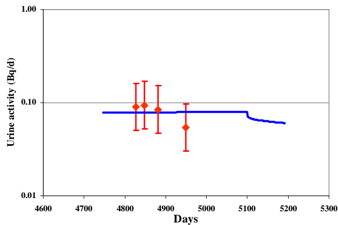
Figure 8-6. Model fit to urine data assuming Type S compound for a chronic intake of 5100 days using only the urine data set for the assessment.
