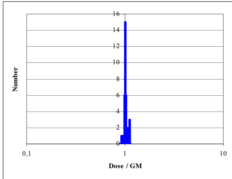
Figure 4-4. Frequency distribution of results without outliers (N=47). Effective dose normalised to the geometric mean. (GM = 25.8 mSv, GSD = 1.06).
